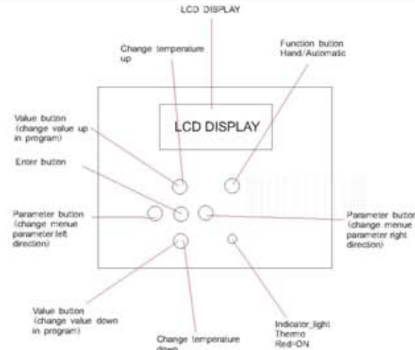
Front Panel
