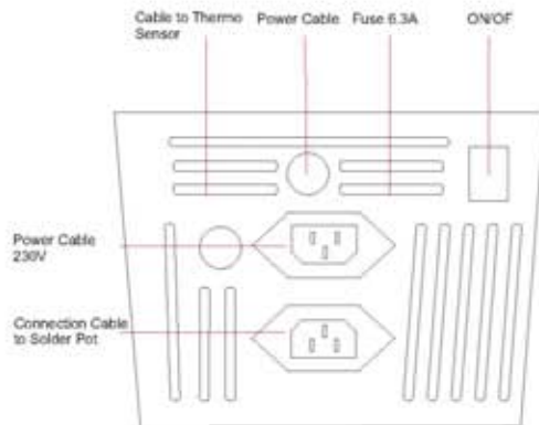
Back Panel
